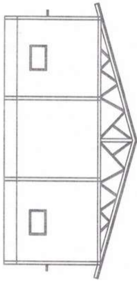
SECTION AT -A'- SCALE 1:100
